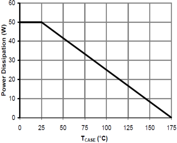
Figure 13: Power De-rating (Note B)
