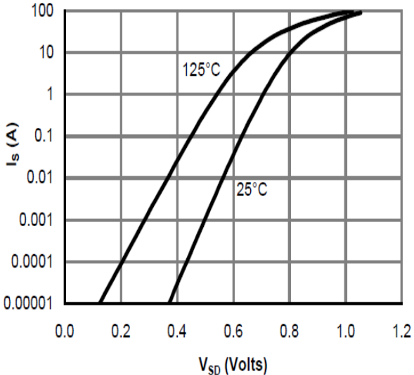
Figure 6: Body-Diode Characteristics
