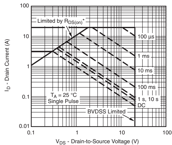
* V_{GS} > minimum V_{GS} at which R_{DS(on)} is specified Figure 12 Safe Operating Area, Junction-to-Ambient
