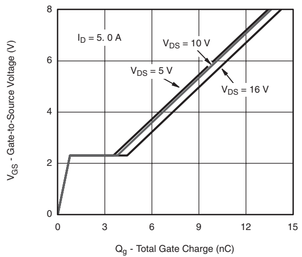
Figure 6 Gate Charge
