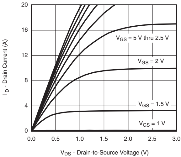
Figure 3 Output Characteristics
