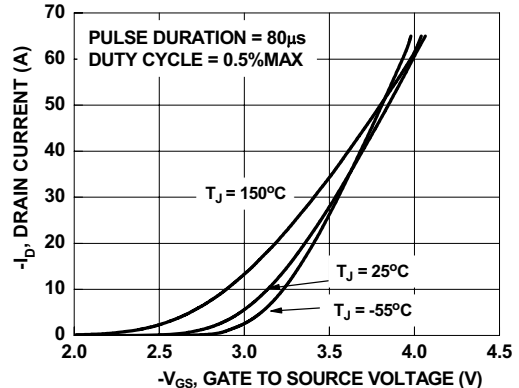
Figure 5. Transfer Characteristics
